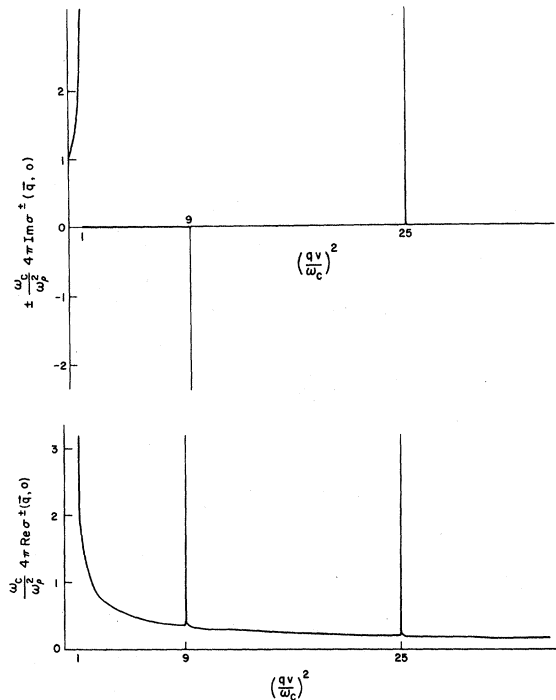
FIG. 1. (a) \pm (\omega_c / \omega_p^2) 4\pi \text{Im } \sigma^*(\vec{q}, 0) and (b) (\omega_c / \omega_p^2) 4\pi \times \text{Re} \sigma^*(\vec{q}, 0) as a function of (qv / \omega_c)^2 for the parameters (43) in the collisionless limit.
